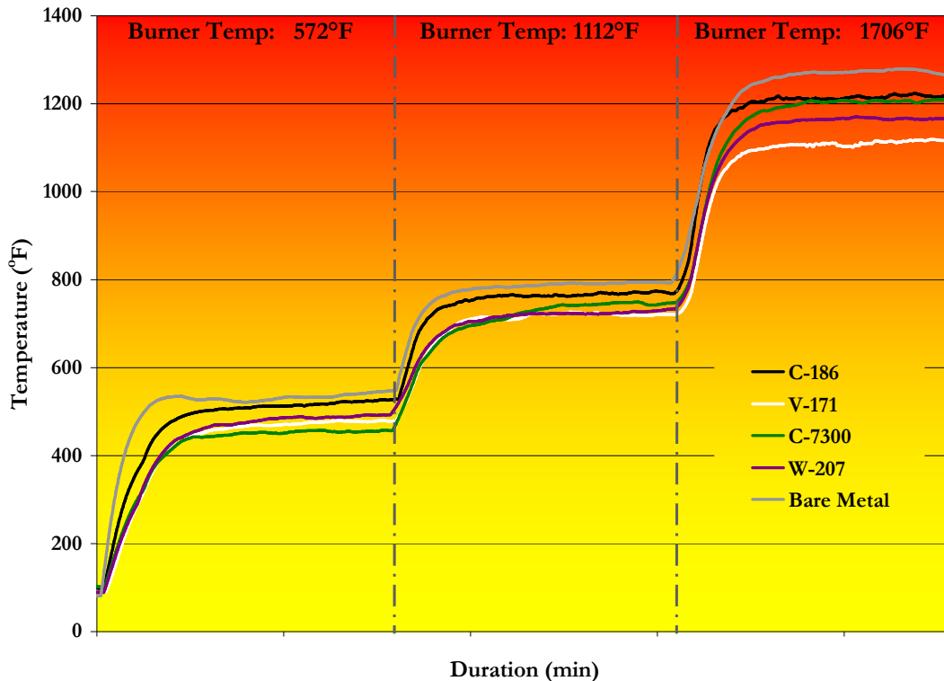
Figure 1. Outer skin temperature profile for 4 pipes coated with Cerakote™ and one uncoated, cold-rolled steel pipe over the temperature range ambient-1706°F.
